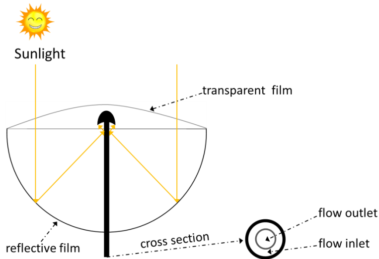
Fig. 1 Solar Receiver Design
