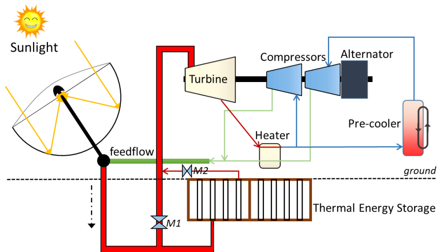
Fig. 3 Schematic of MCSP-ED
